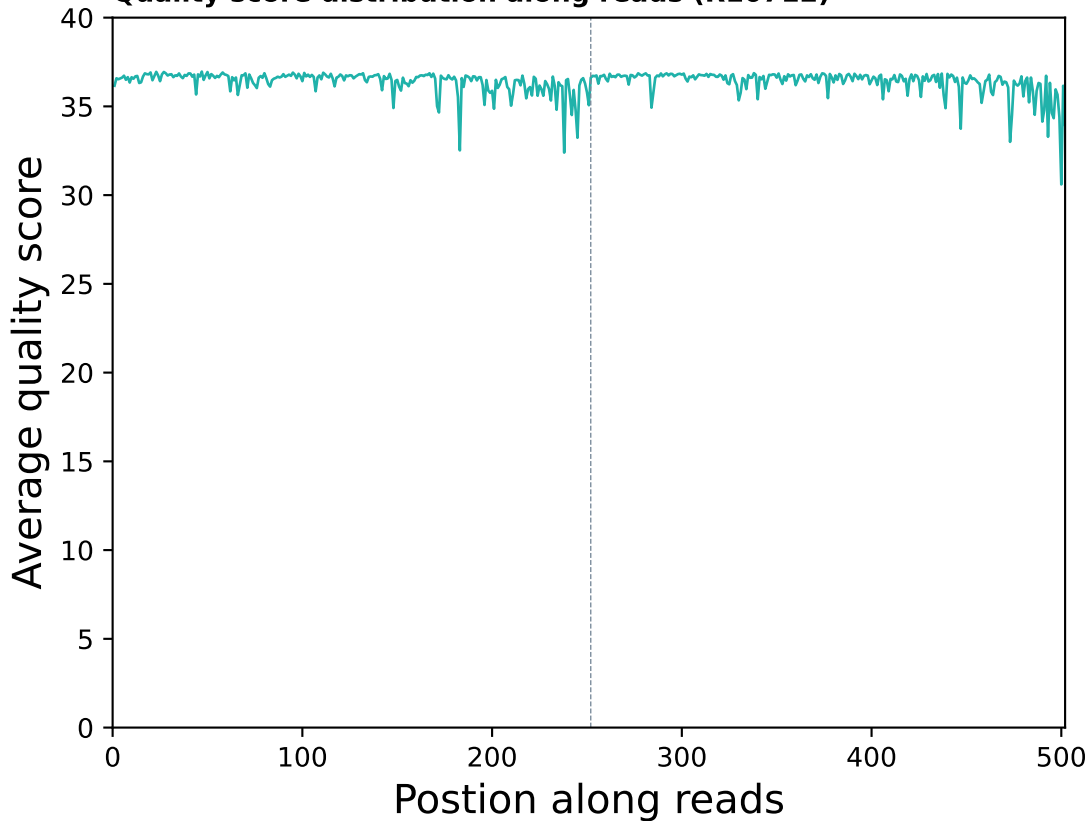
Quality score distribution along reads (R10712)
